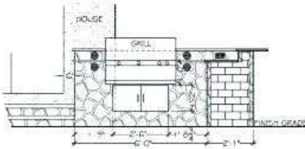
KITCHEN - EAST VIEW SECTIONAL ELEVATION BB
