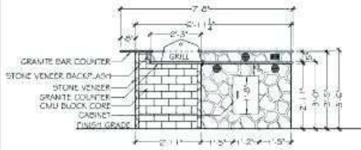
KITCHEN - NORTH VIEW SECTIONAL ELEVATION AA
